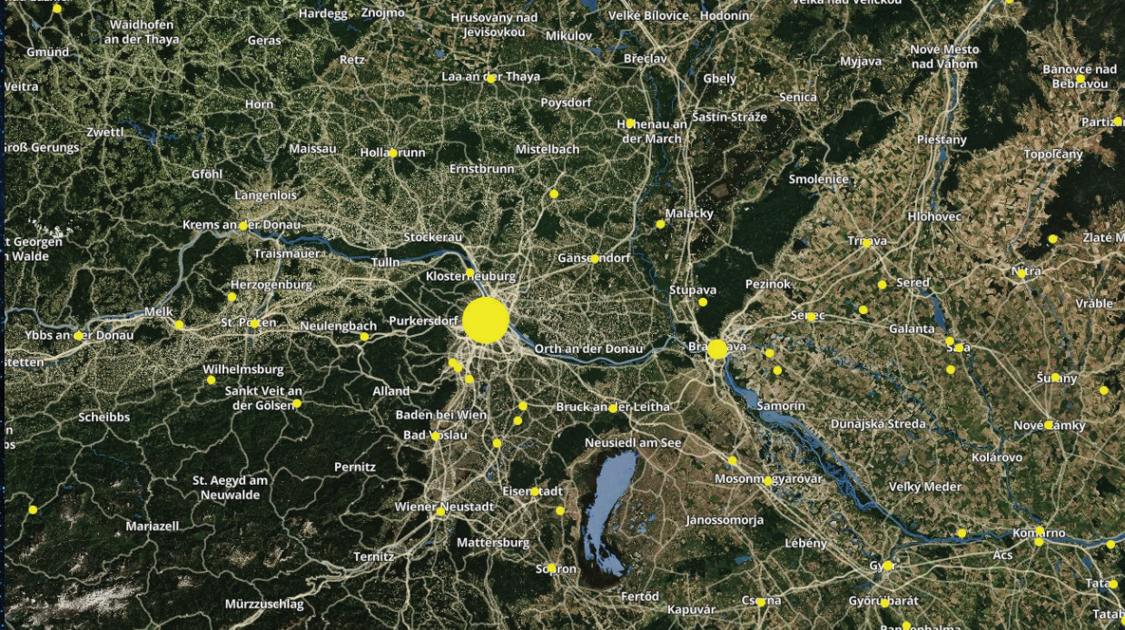
Map of Asgardians, view from Vienna, Austria
